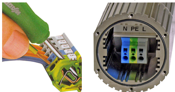
Protected Side, cover with cable gland removed
